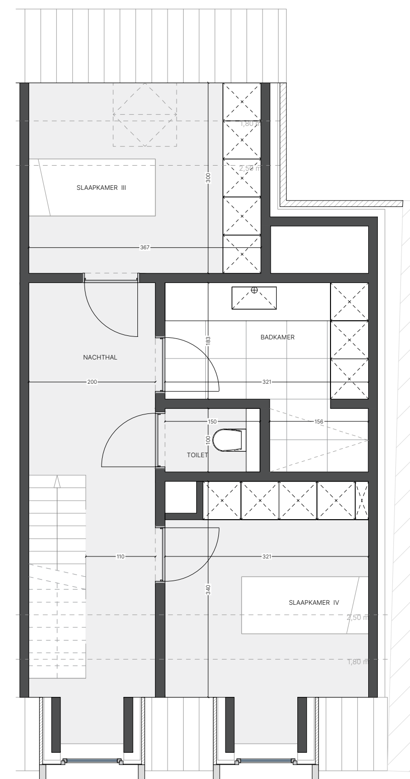
ZOLDER
